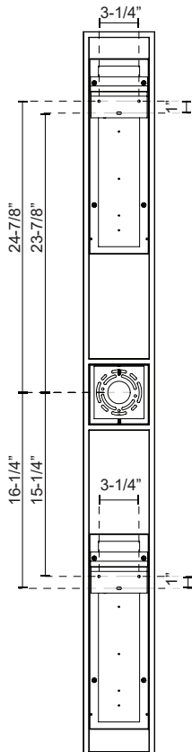
Illustration 2: Ideal distance of non-power mounting plate to mounting plate and ideal distance of anchor holes.
