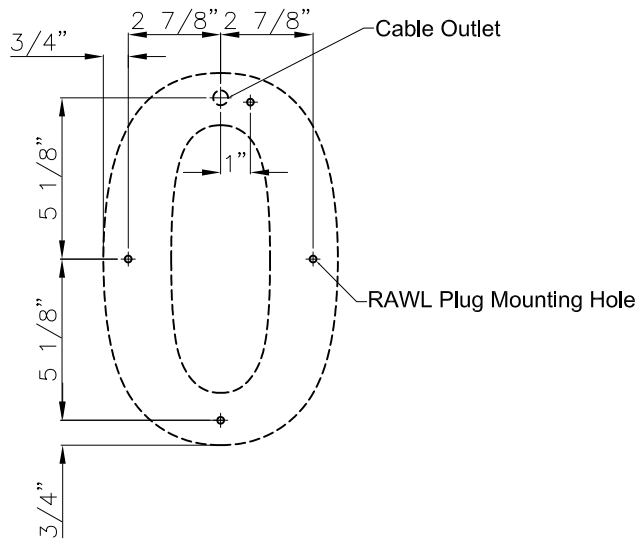
Mounting Screws Diagram
