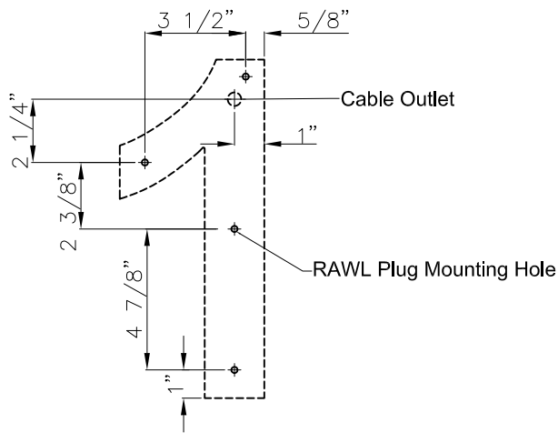
Mounting Screws Diagram
