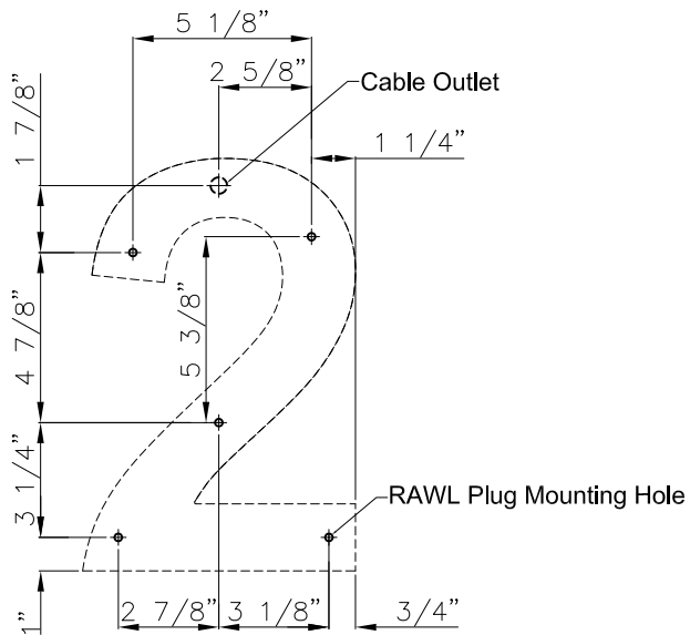
Mounting Screws Diagram
