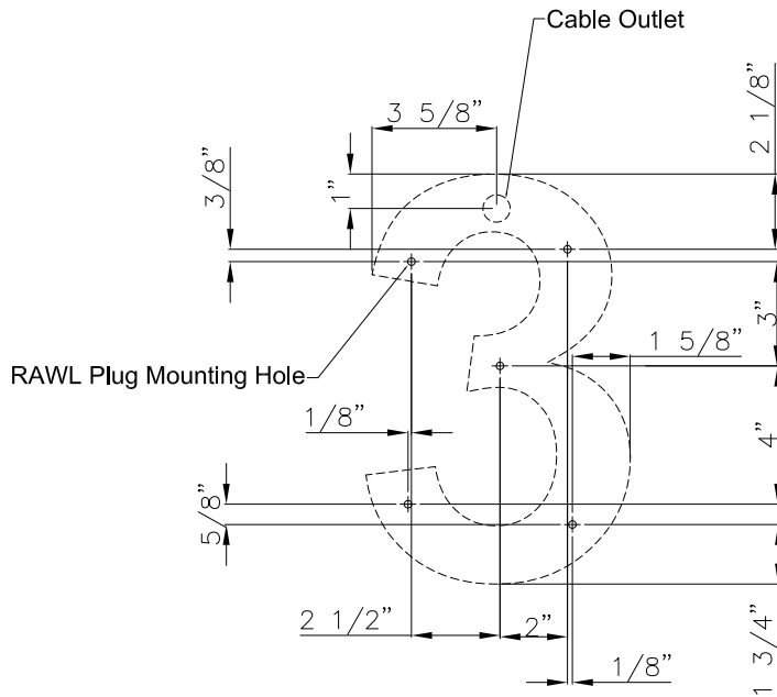
Mounting Screws Diagram
