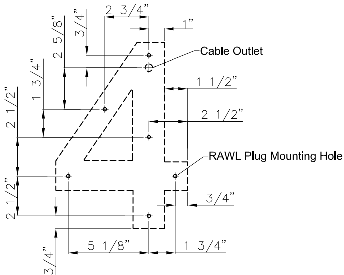
Mounting Screws Diagram
