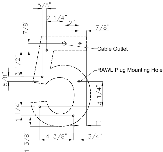
Mounting Screws Diagram
